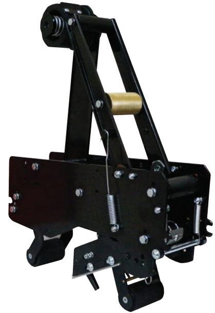
Shown Above is the BestPack TH High Speed Tape Head with Optimizing Arm and a Unique 5 Roller Tape Feed System.
