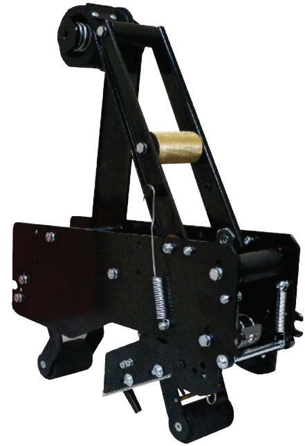
Shown Above is the BestPack TH High Speed Tape Head with Optimizing Arm and a Unique 5 Roller Tape Feed System.
