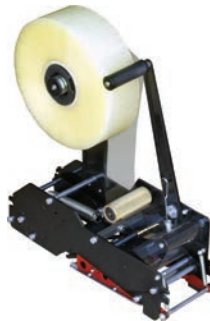
3" TAPE HEAD
